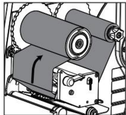
Ribbon Take-up Spindle
